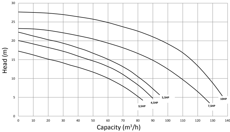
Performance Curve
